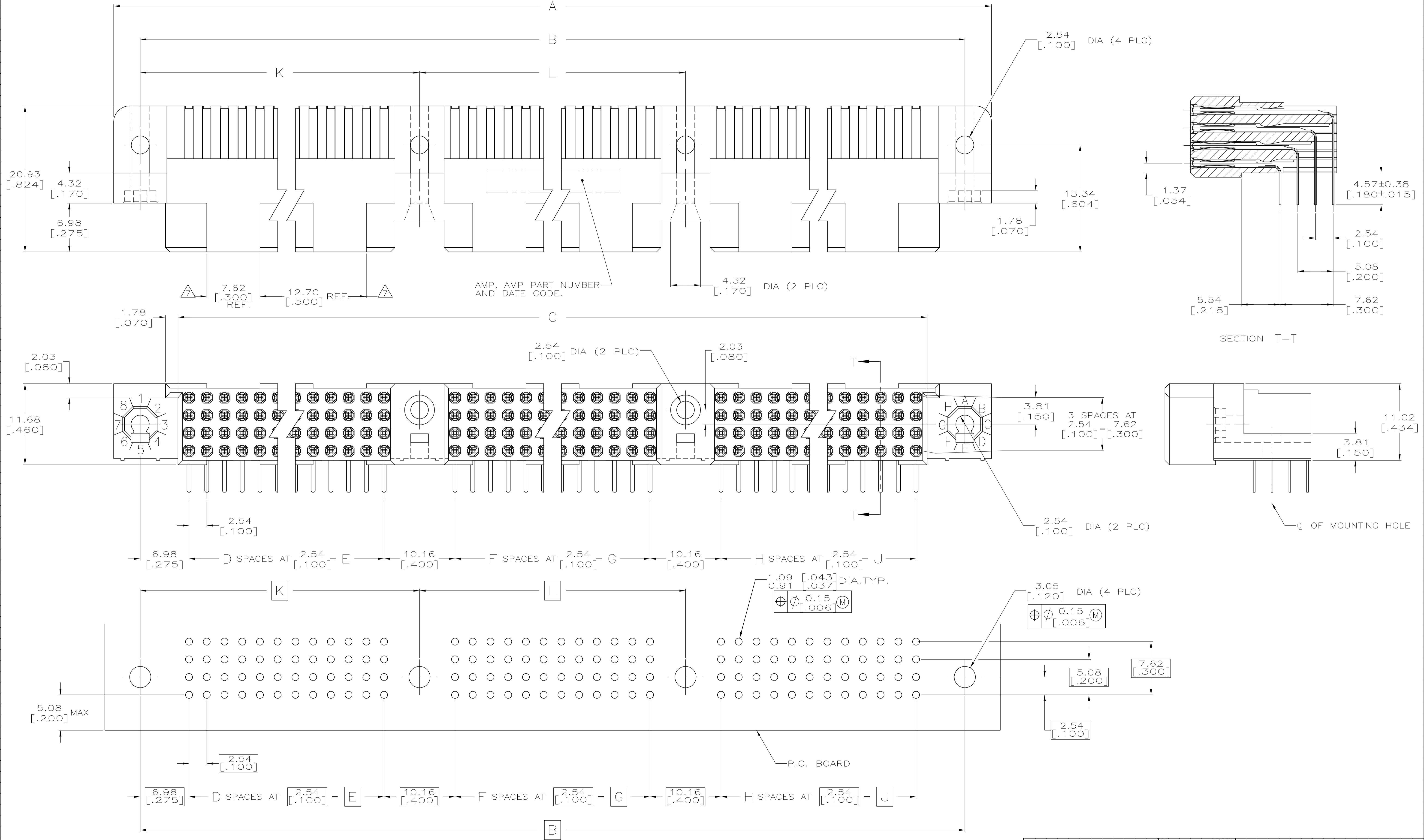
RECOMMENDED P.C. BOARD LAYOUT
